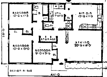
A SMALL HOUSE PLANNING BUREAU DESIGN NO. A-546
